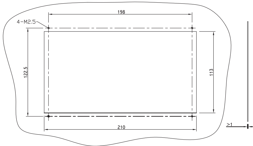
INDICATOR MOUNTING DIMENSION
